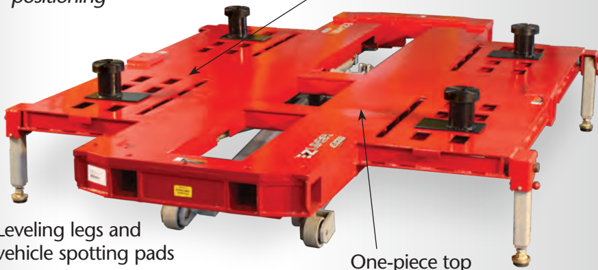
Tall anchor clamps allow compatibility with all Chief computerized measuring systems - anchors and clamps included
